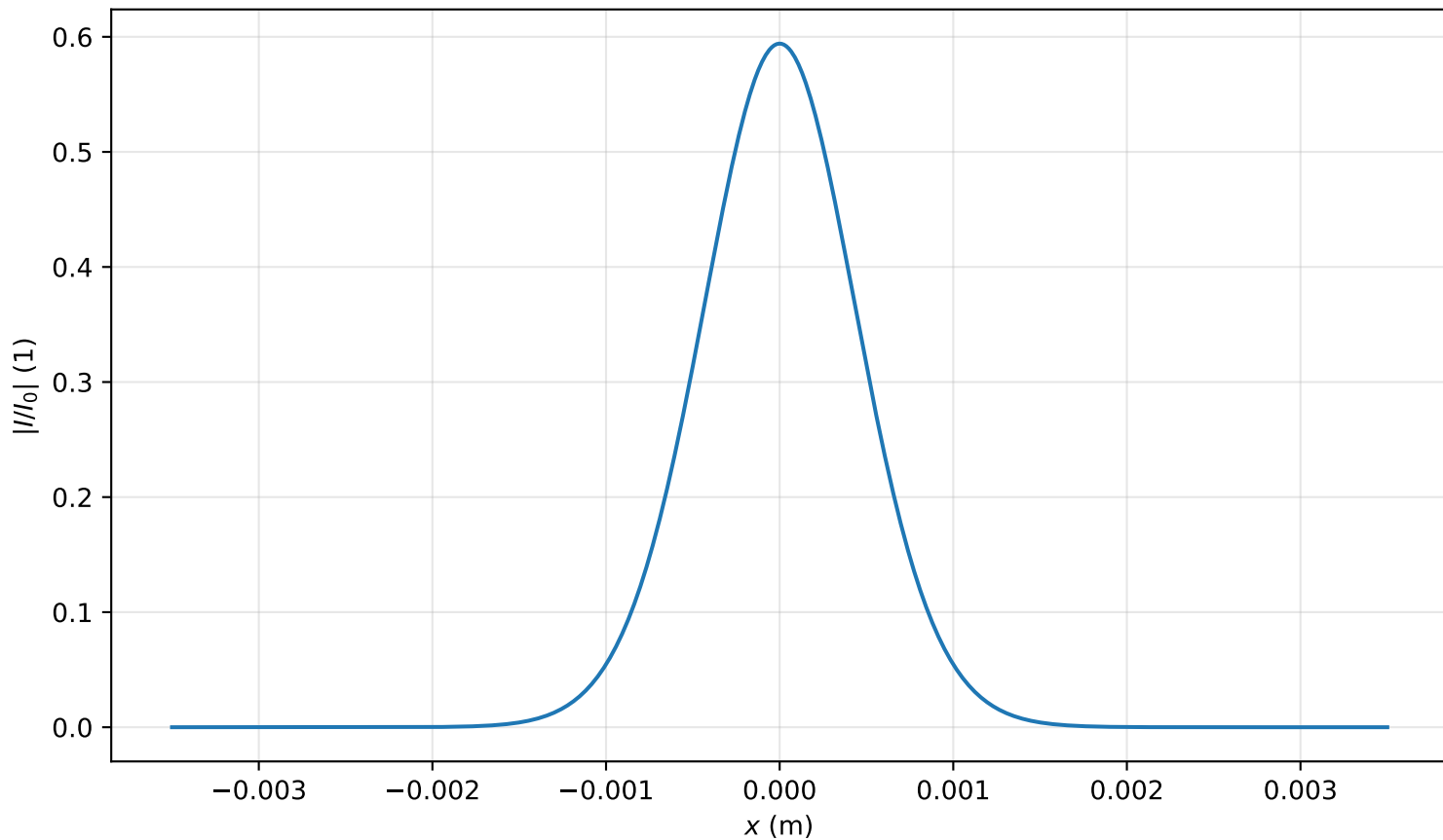
Intensity profile I(x, y = 0, z = 1.990m)/I_0 , P_{in}=0.2P_{cr} , artificial time
